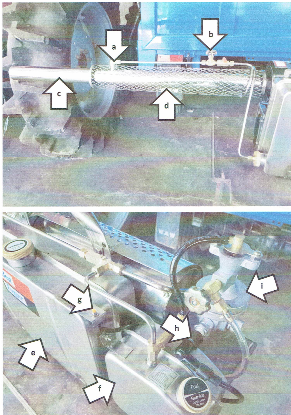
Figure 1. Parts of the BEST FOGGER BF150 Automatic Fogging Machine: (a) Chemical nozzle, (b) Chemical control valve, (c) Fogger outlet, (d) Fogger outlet safety cover, (e) Chemical tank, (f) Fuel tank, (g) Start button, and (h) Spark plug.
